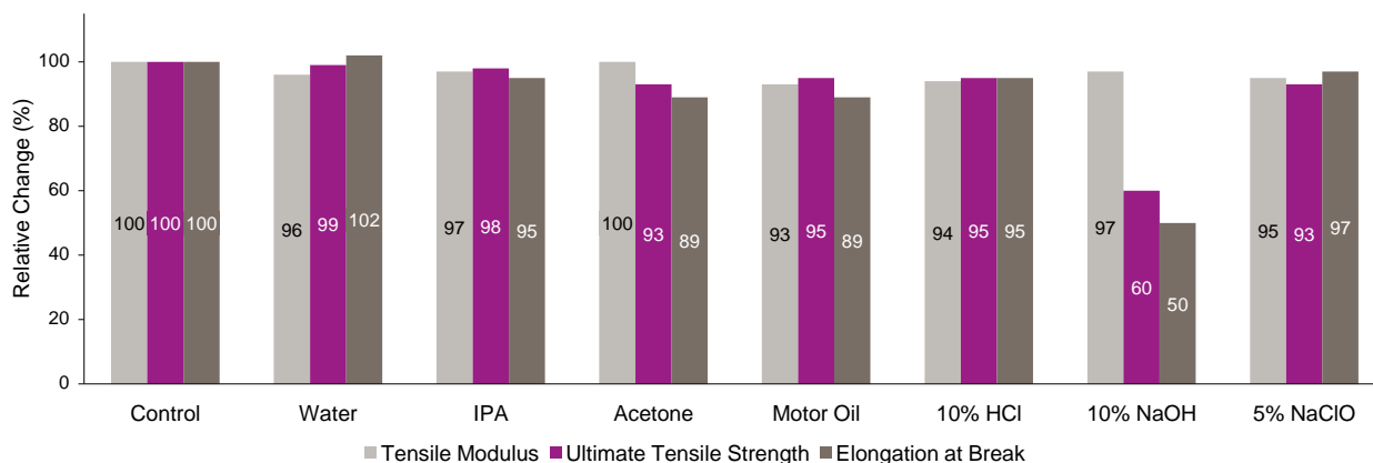
Retained tensile properties in % after 24 h immersion in test liquids
