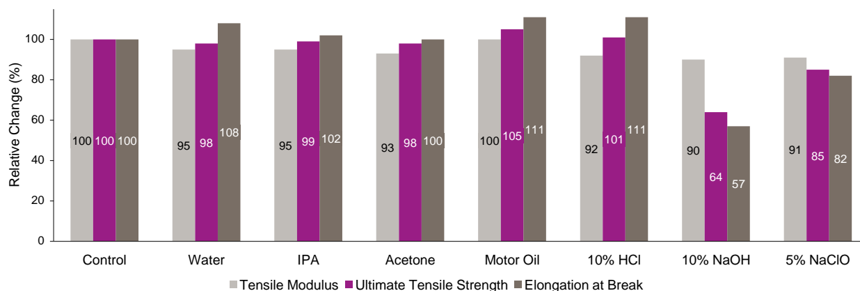
Retained tensile properties in % after 7 days immersion in test liquids
